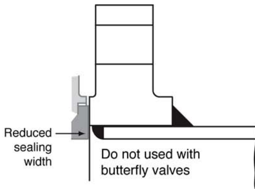
Slip On Welding Flange
