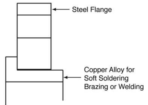
Loose Plate Flange with Slip On Collar
