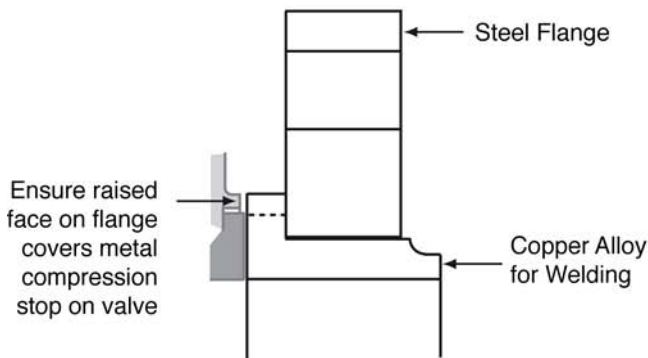
Loose Plate Flange with Weld Neck Collar
