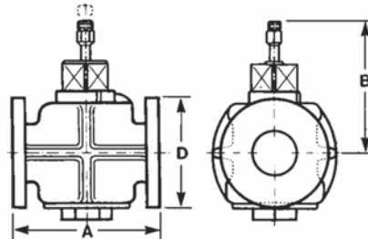
Fig. 201R - Sizes 1 1/4" to 4" 4" size has bolted bottom cover
